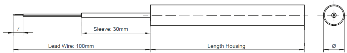
Cartridge Heater PSS 110-240V
